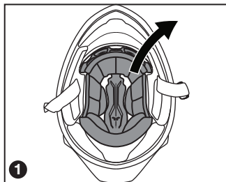
1 REMOVE THE INNER LINING
